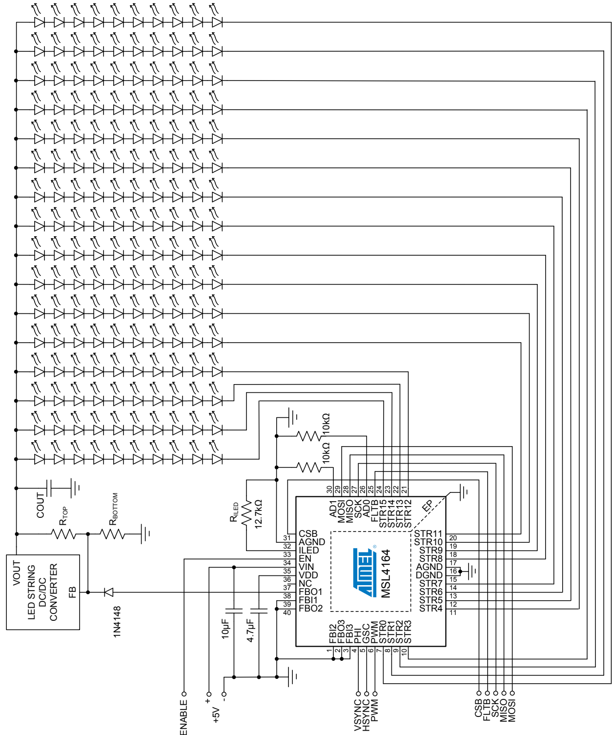
Figure 5. Atmel LED Driver-MSL4164 Driving 160 White LEDs in 16 Strings at 60mA per String.
