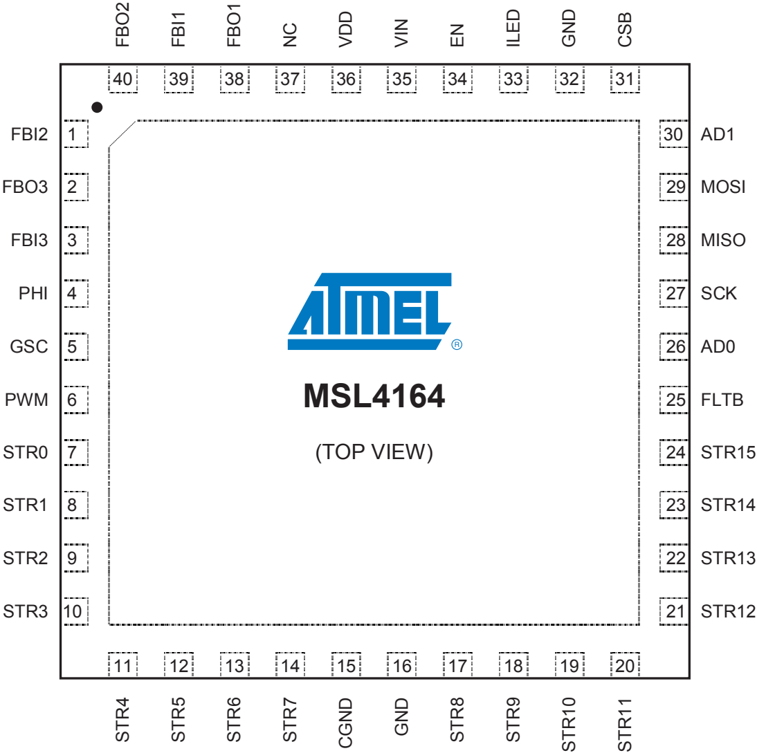
Figure 2. Atmel LED Driver-MSL4164 Pin-out, 40-pin TQFN.
